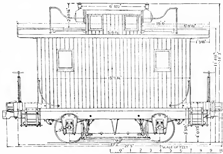
Fig. 81. Side Elevation.
